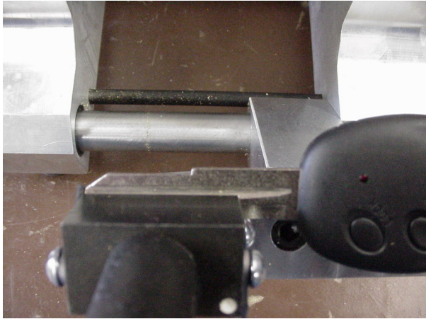
Figure 1. Inserting the key into the non-dot side of the vise
